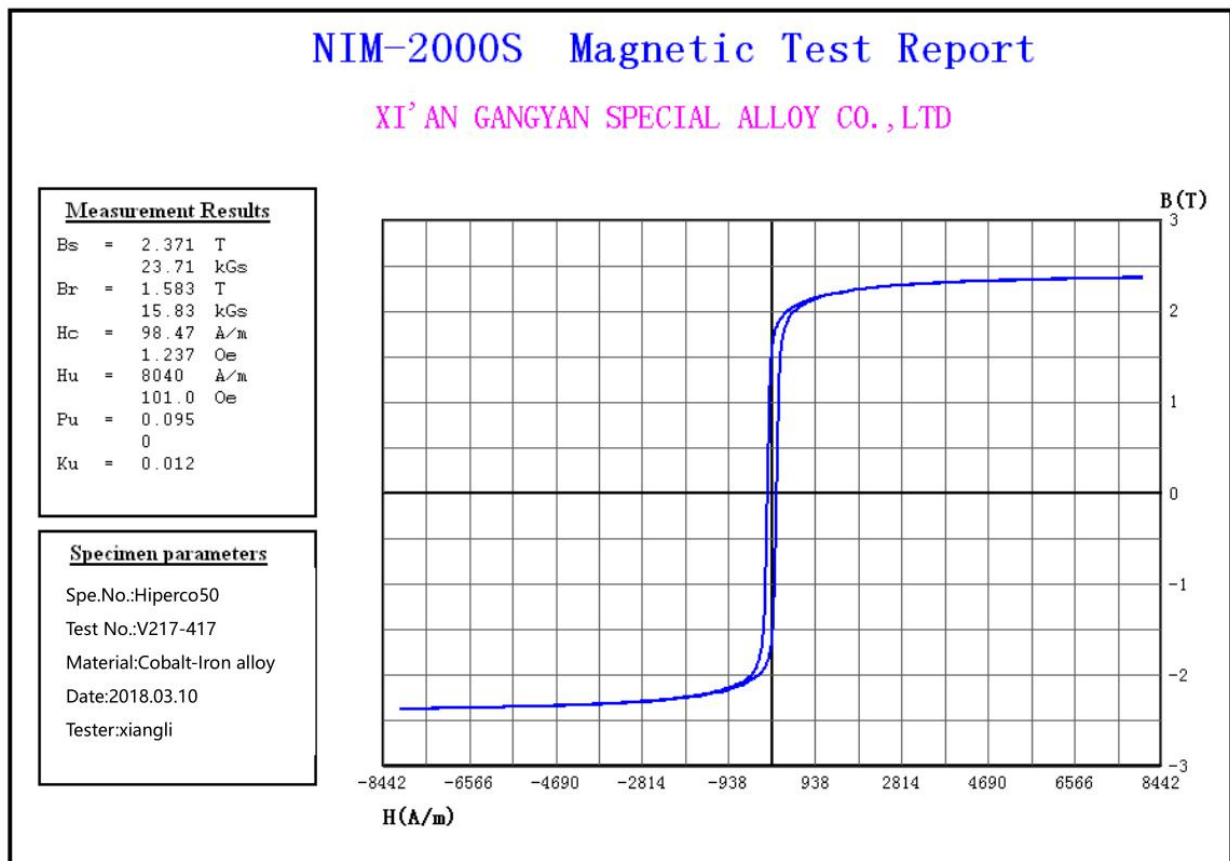
Hysteresis loop curve of Hiperco 50 (Dia.100.0 mm)
