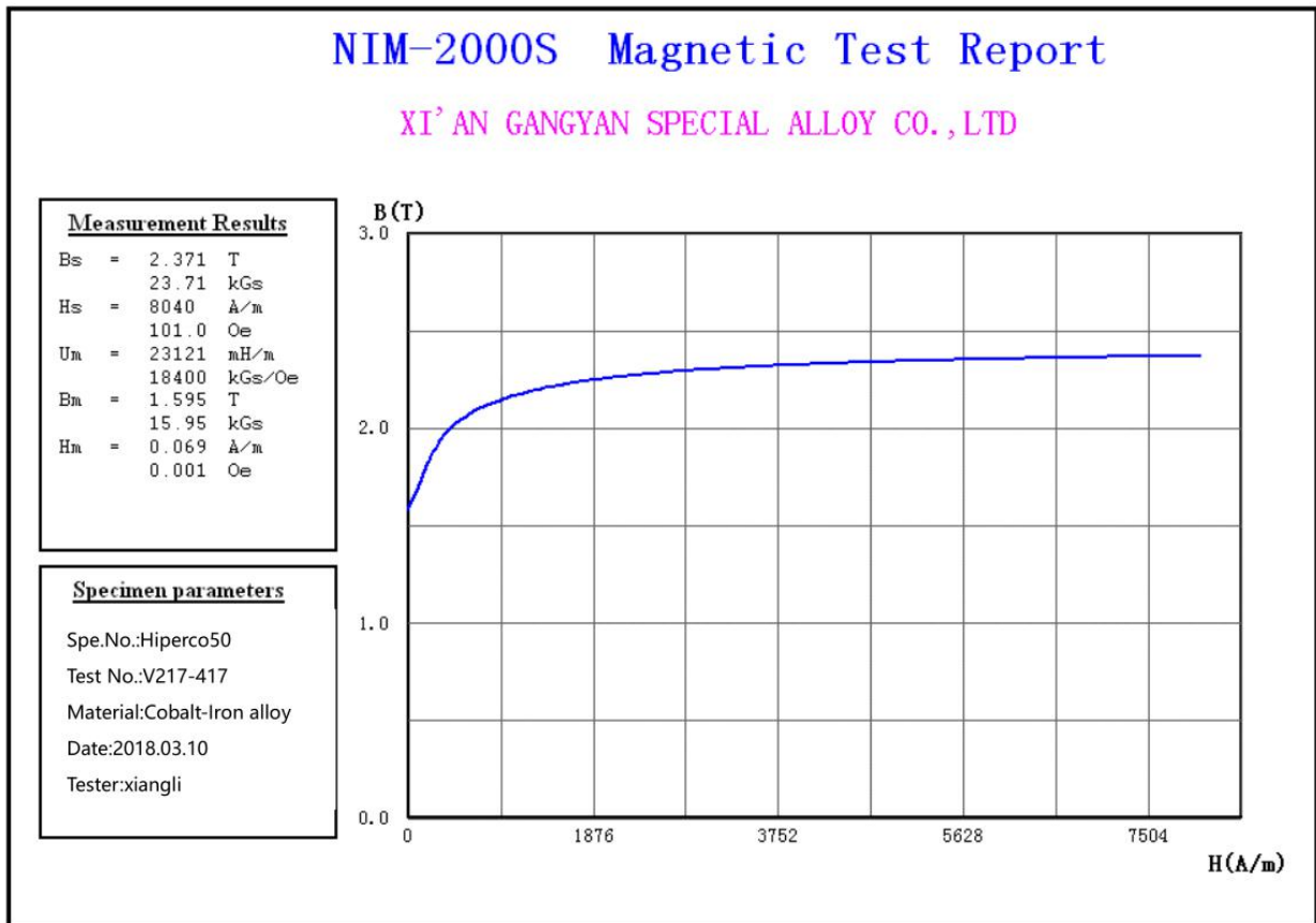
Magnetization curve of HiperCo50 (Dia.100.0 mm)
