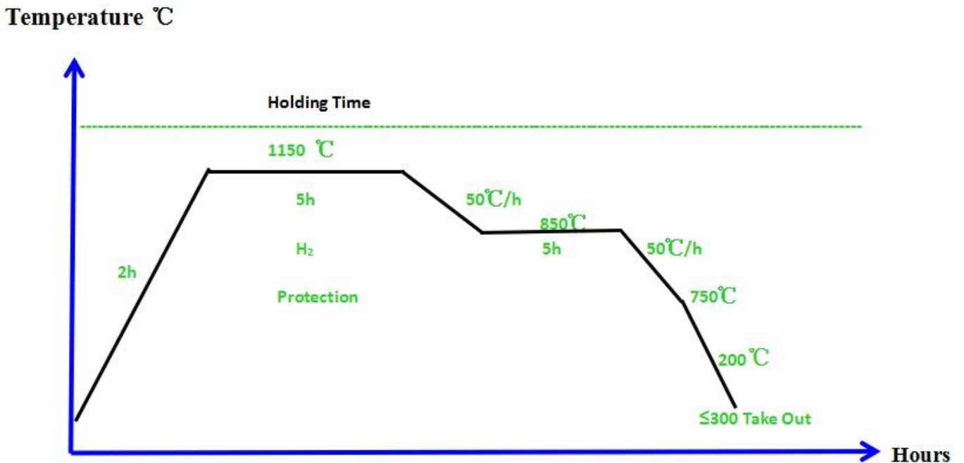
Recommending Heat Treatment Method for Hipercro 50 Rod/Plate (Components)
