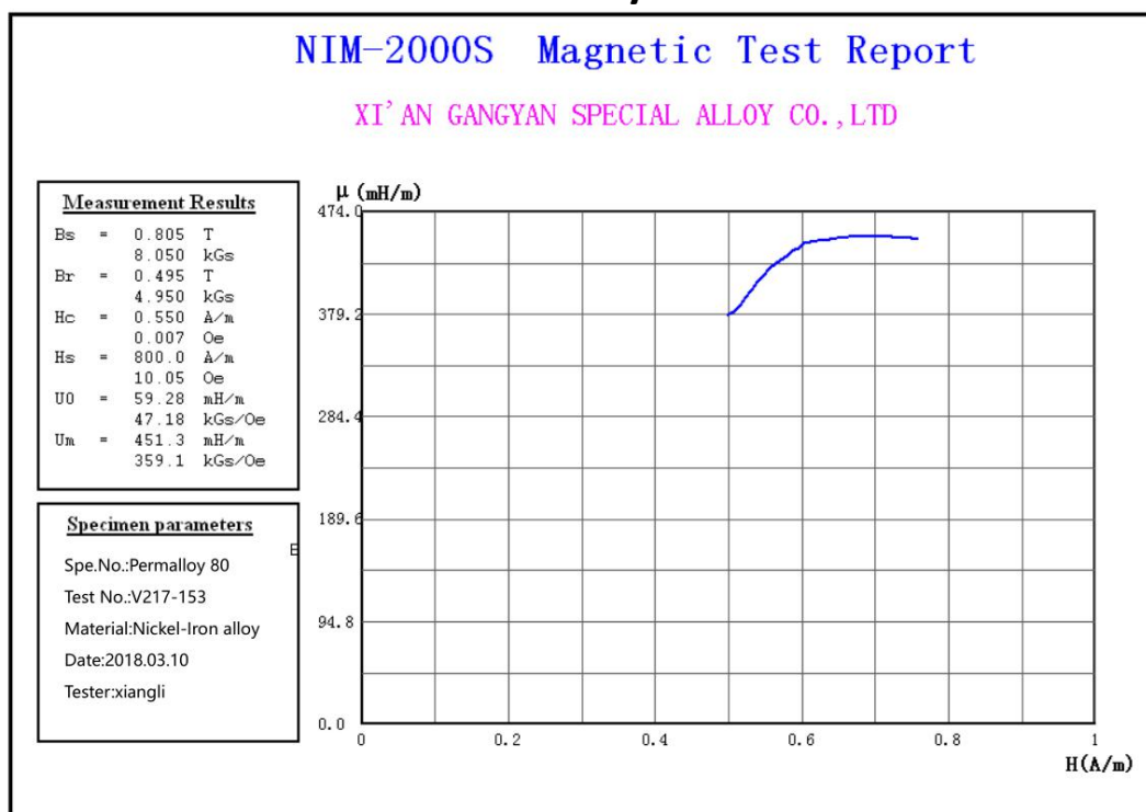
Permeability curve of Permalloy 80 ( \delta=1.0\text{mm} )
